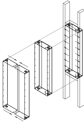
Wood stud configuration Add framing above and below.
